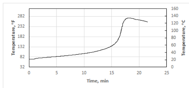
Typical Exotherm Curves for MA805 in 10 g Mass at 74 °F (23 °C) 5
